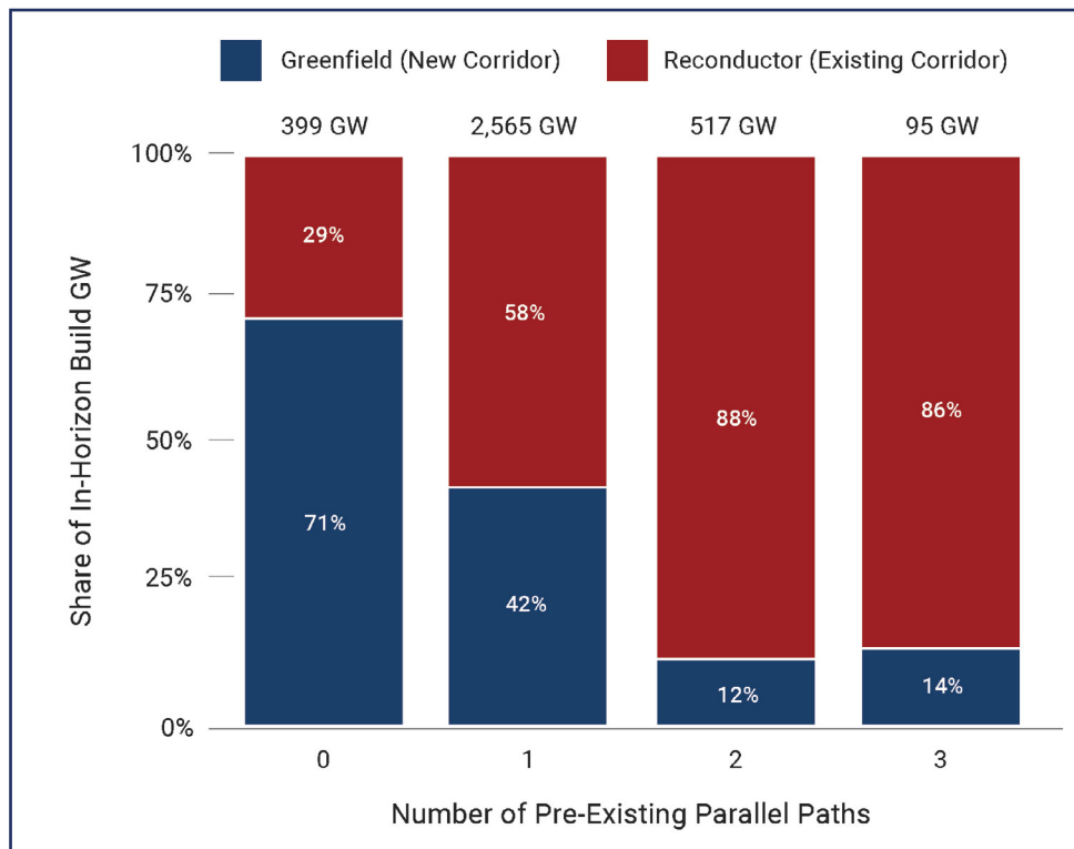
Figure 9. Pre-existing parallel paths are a predictor of whether reconductoring or a greenfield expansion approach is the most cost-effective way to expand the system while maintaining reliability.
